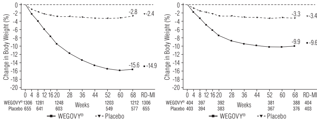
Figure 6. Change from Baseline (%) in Body Weight (Study 1 on Left and Study 2 on Right)
