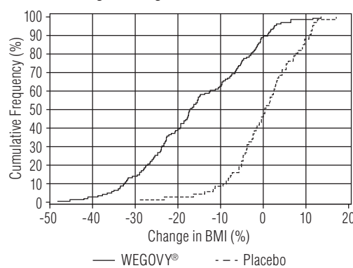
Figure 9. Change in BMI (%) from Baseline to Week 68 in Pediatric Patients with Obesity Aged 12 Years and Older in a Weight Management Trial
